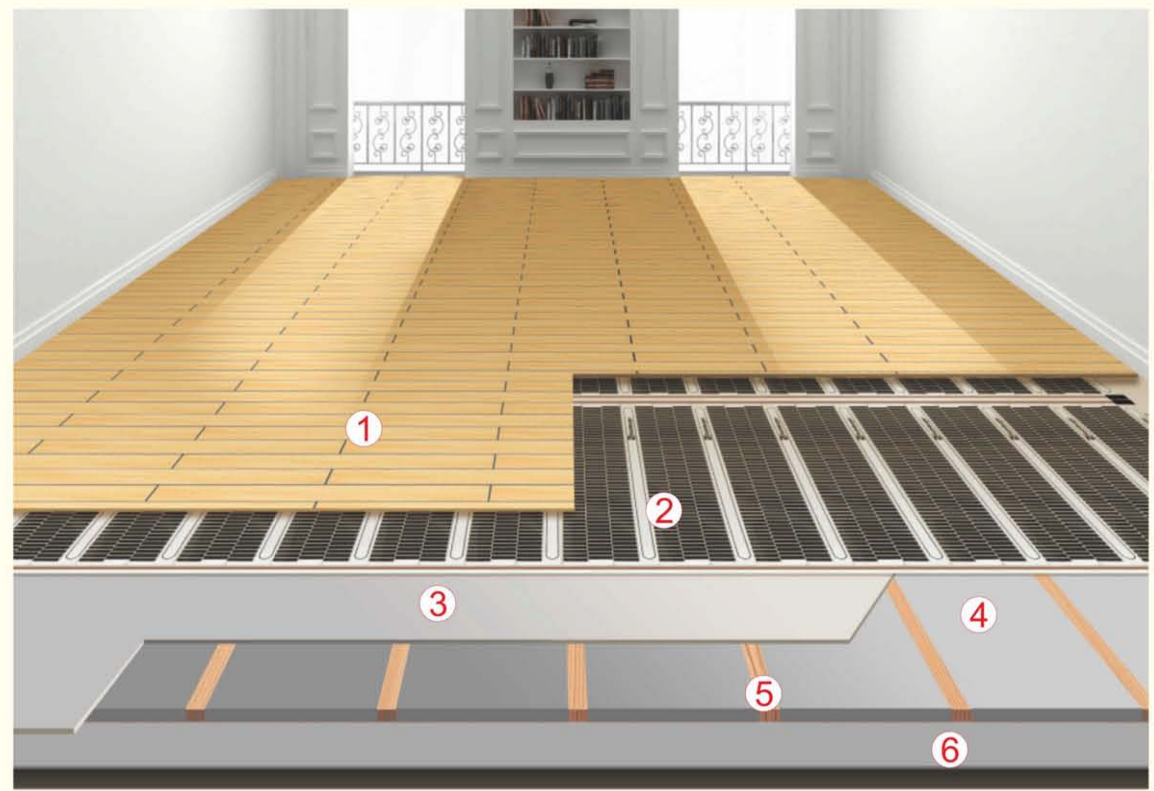
①Wood flooring ②MPTC ③IXPE insulation film ④Insulation mortar ⑤Wood keel ⑥Foundation
